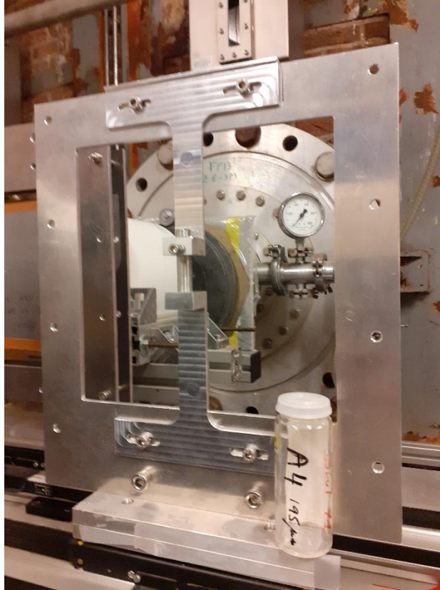
Figure 1. One of the MINERVE samples at GELINA FP13-10 station
