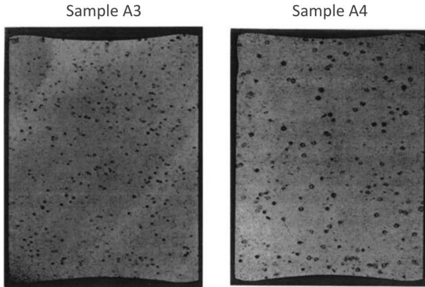
Fig. 1. Micrography of two \text{UO}_2 pellets containing microspheres of \text{Gd}_2\text{O}_3 of 120 and 195 \mu\text{m} .
