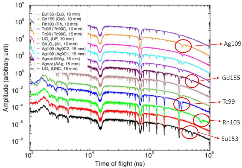
Fig. 3. Examples of raw data obtained with MINERVE samples containing ^{107}\text{Ag} , ^{155}\text{Gd} , ^{99}\text{Tc} , ^{103}\text{Rh} and ^{153}\text{Eu} isotopes.
