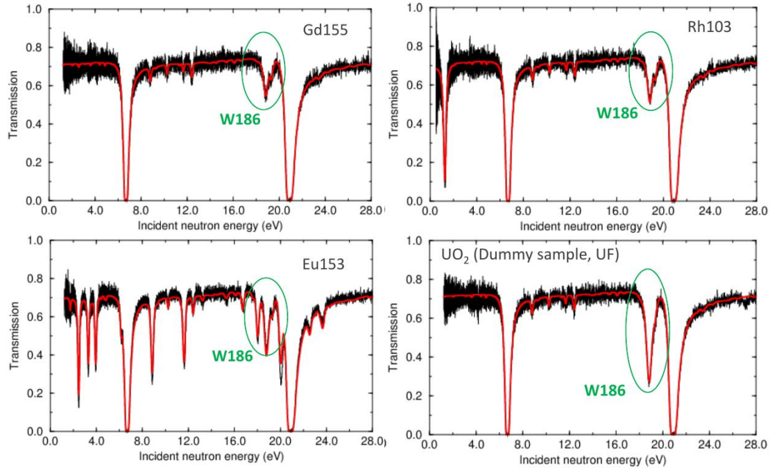
Fig. 4. Examples of tungsten contamination observed in MINERVE samples. The solid curves represent the theoretical transmission calculated with the REFIT code.
