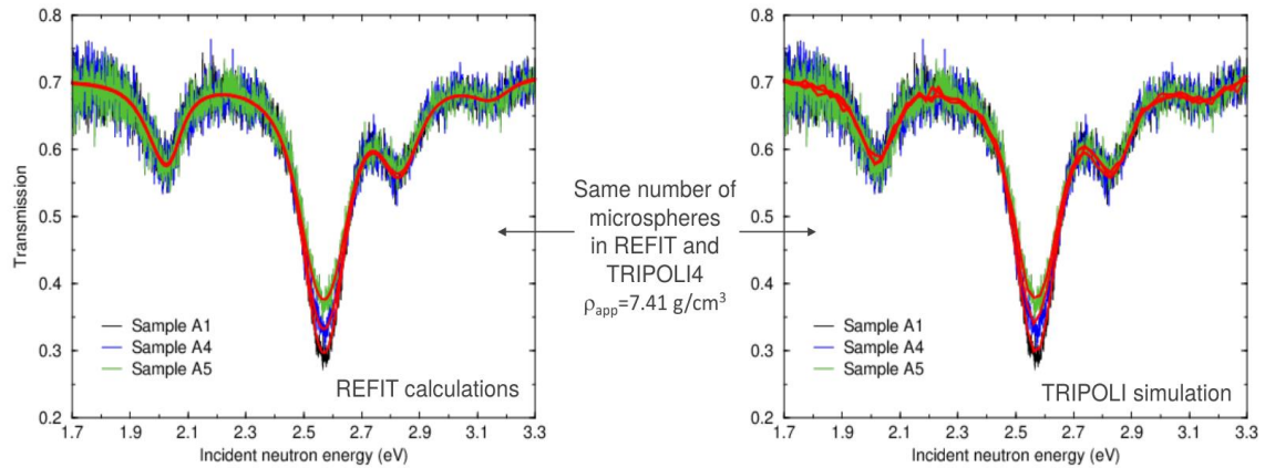
Fig. 5. Examples of transmission data obtained around the ^{155}\text{Gd} resonance at 2.6 eV by using MINERVE samples coming from the GADOLINIUM program. Each sample contains the same amount of \text{Gd}_2\text{O}_3 . In sample A1, gadolinium oxide powder is homogeneously mixed with the \text{UO}_2 matrix. In samples A4 and A5, the diameter of the microspheres of \text{Gd}_2\text{O}_3 is close to 195 and 380 \mu\text{m} , respectively. The same number of microspheres were used in the REFIT and TRIPOLI calculations.
